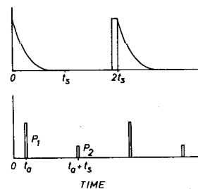
FIG. 3. Typical time sequence for afterglow noise sampling. The upper part represents the plasma noise emission during breakdown pulse and afterglow. The lower picture shows the radiometer's noise power samples. For each breakdown period ( 0 < t < 2t_s ) a signal sample ( P_1 ) and a reference sample ( P_2 ) are taken.
