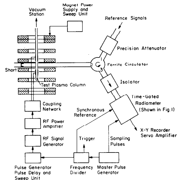
FIG. 2. Block diagram of the main elements for sampling and comparison measurements on a magnetized afterglow plasma column.
