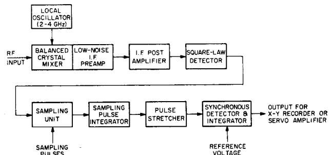
FIG. 1. Block diagram of the time gated radiometer.
