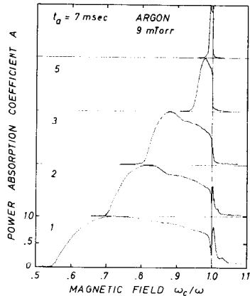
FIG. 4. Power absorption coefficient vs normalized magnetic field at different times in the afterglow. The upper hybrid resonances lie in the range (1 - \omega_{pmax}^2/\omega^2)^{1/2} \leq \omega_c/\omega \leq 1 . The narrow absorption line at \omega_c/\omega \geq 1 is a side effect due to the fringing fields of the holes in the waveguide sidewalls.
