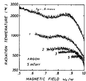
FIG. 7. Electron temperature vs normalized magnetic field at different times in the afterglow. The variation is due to the shift of the upper hybrid resonance from the center of the column to the wall and thus reflects the spatial temperature variation. The temperature can be measured only in the range of nonzero absorption, i.e., in the hybrid frequency range.
